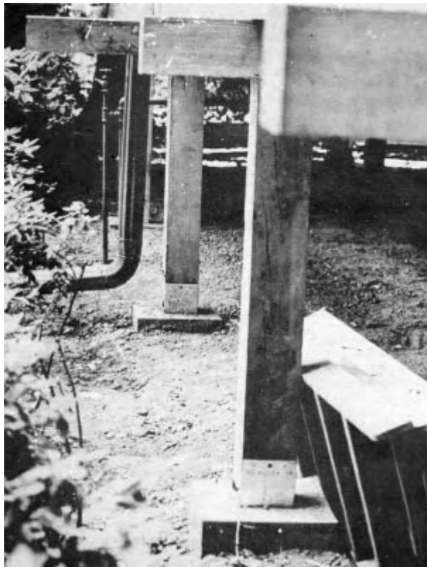
Figure 6. New posts are in place. The post-anchors will reduce future water damage.
