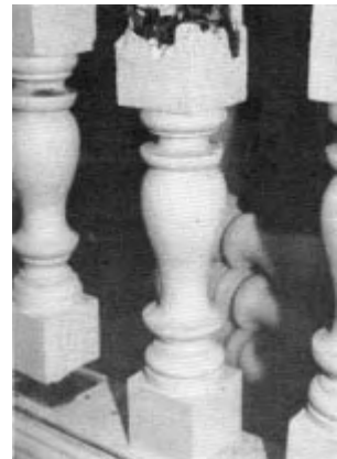
Figure 8. Balusters decay at block ends. Cut off these ends and repair with a doweled block to save the expense of turning new balusters.
